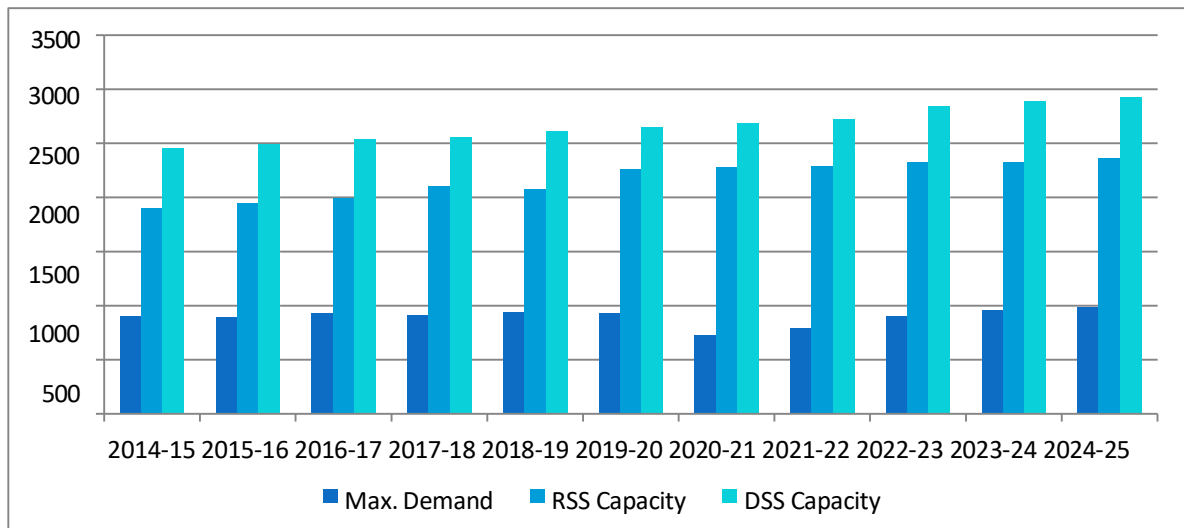
Figure 1 Maximum Demand of BEST in MVA and Installed Capacity of RSS (MVA) and DSS (MVA)
